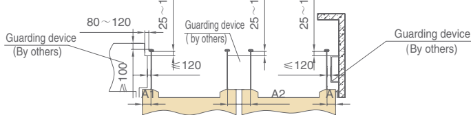
Guarding device at access
